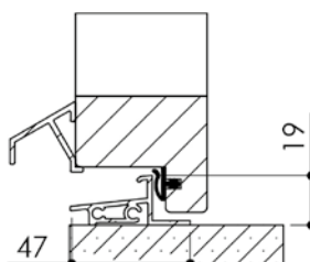
Seuil alu PMR Version Residence C
