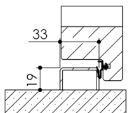
Seuil U inversé Version Residence P
