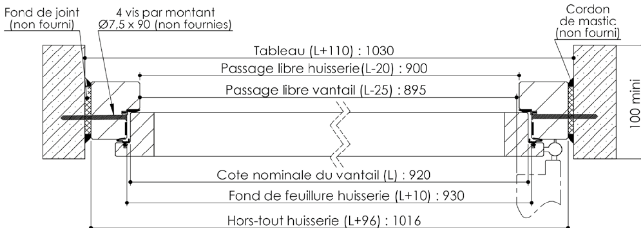
Seuil alu PMR Version Residence C
